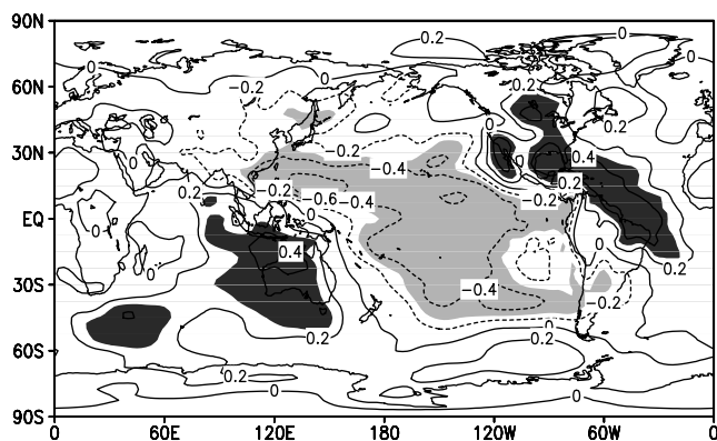
Figure 6. Horizontal distribution of the correlation coefficient between the seasonal (June–September) sea level pressure anomalies and SCSSMI for the period 1958–97. Critical positive (negative) values of the correlation at the 95% confidence level are shaded dark (light). The map shows that global shifts of atmospheric mass take place during strong South China Sea summer monsoon anomalies period.
