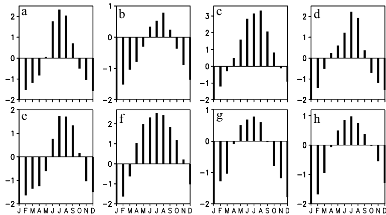
Figure 1. Seasonal variation of the DNS index calculated in the eight key monsoon sectors of (a), South Asian ( 5^{\circ} – 22.5^{\circ} N, 35^{\circ} – 97.5^{\circ} E) at 850hPa, (b), East Asian ( 10^{\circ} – 40^{\circ} N, 110^{\circ} – 140^{\circ} E) at 850hPa, (c), South China Sea ( 0^{\circ} – 25^{\circ} N, 100^{\circ} – 125^{\circ} E) at 925hPa, (d), African ( 5^{\circ} – 17.5^{\circ} N, 20^{\circ} W– 40^{\circ} E) at 850hPa, (e), North American ( 17.5^{\circ} – 35^{\circ} N, 100^{\circ} – 120^{\circ} W) at 700hPa, (f), Australian ( 5^{\circ} – 20^{\circ} S, 100^{\circ} – 160^{\circ} E) at 925hPa, (g), South American ( 10^{\circ} – 17.5^{\circ} S, 50^{\circ} – 62.5^{\circ} W) at 925hPa and (h), Southern Equatorial West Indian Ocean ( 0^{\circ} – 20^{\circ} S, 37.5^{\circ} – 50^{\circ} E) at 925hPa for the period 1979–99.
