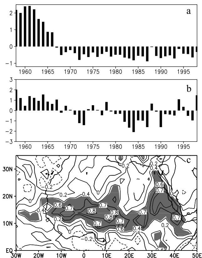
Figure 3. Normalized time series of ASMI (a) and summer rainfall (June–September) over the West African Sahel ( 12.5^{\circ} – 17.5^{\circ} N, 20^{\circ} W– 30^{\circ} E) from Hulme [Hulme et al. , 1998] (b) for the period 1958–98. (c), Correlations between the seasonal (June–September) rainfall from the Xie-Arkin rainfall analysis [Xie and Arkin, 1997] and DNS index for the ASM (1979–97). Critical positive (negative) values of the correlation at the 95% confidence level are shaded dark (light).
