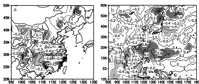
Figure 4. Correlations between the seasonal (June–August) East Asia index and (a), precipitation over China (1958–99), and (b), precipitation over the East Asia from the Xie-Arkin rainfall analysis [Xie and Arkin, 1997] (1979–97).
