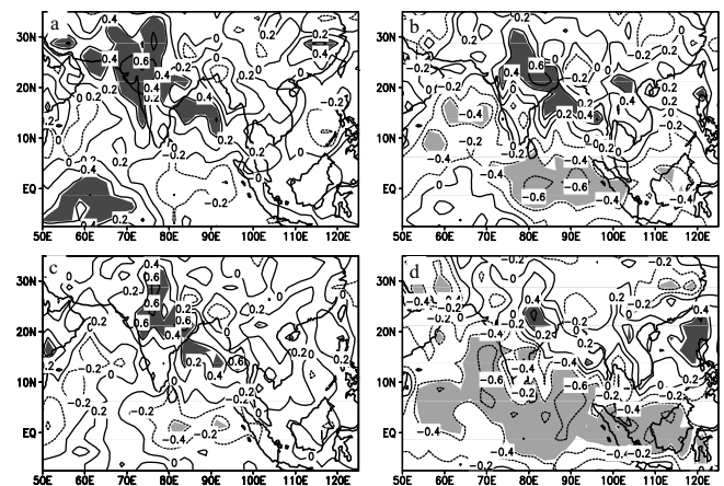
Figure 2. Correlations between the seasonal (June–September) rainfall and (a), AIRI, (b), SASMI, (c), SASMI1, and (d), SASMI2 for the period 1979–97. Critical positive (negative) values of the correlation at the 95% confidence level are shaded dark (light).
