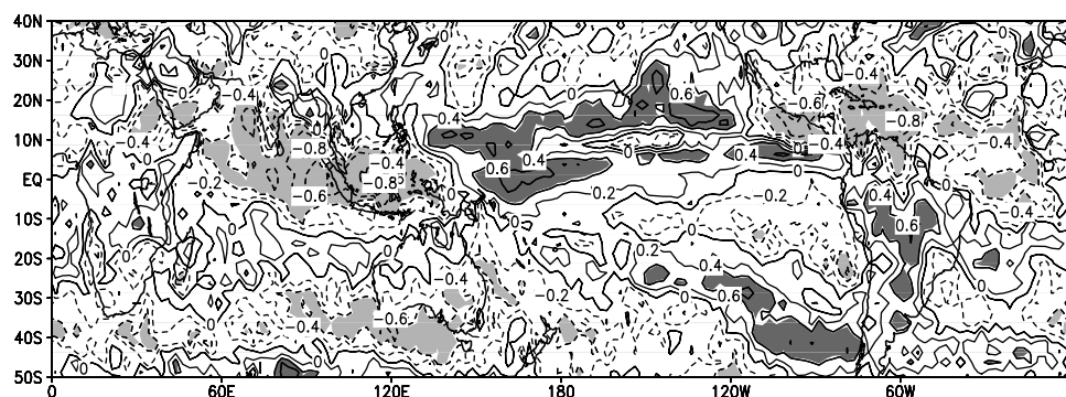
Figure 5. Correlations between the seasonal (June–September) rainfall and SCSSMI. Critical positive (negative) values of the correlation at the 95% confidence level are shaded dark (light). The period is for 1979–97.
